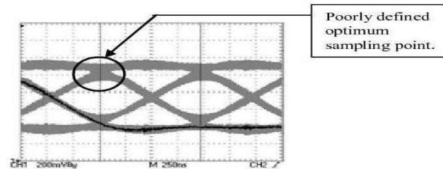
Figure 12-4. Distorted eye diagram
