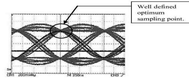
Figure 12-3. Ideal eye diagram
