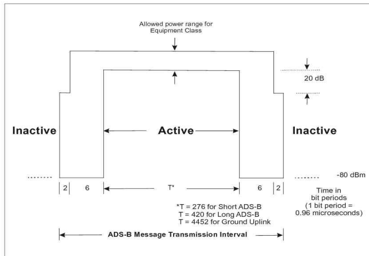
Figure 12-2. Time/amplitude profile of UAT message transmission
